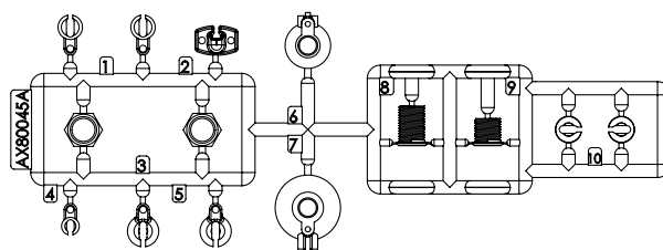
AX80045 (x2) Light Bucket Set (Black) Lichtschalen-Set (schwarz) Ensemble de spots lumineux (noir) Set corpo fanale (nero)
